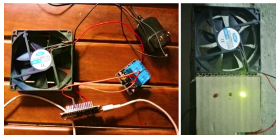
Fig. 5. Control System Integration.
