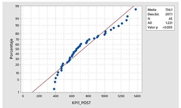
Fig. 10. Normality Test KPII Post-Test.
